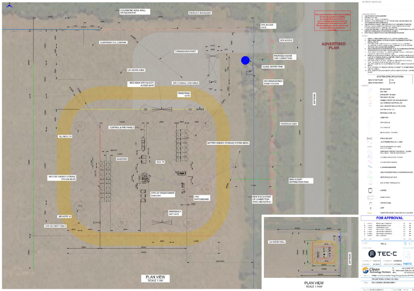
Figure 42: PICES battery site arrangement
